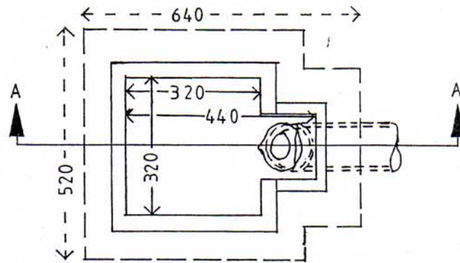
PIT PLAN (BUCKET & PLATE REMOVED)
